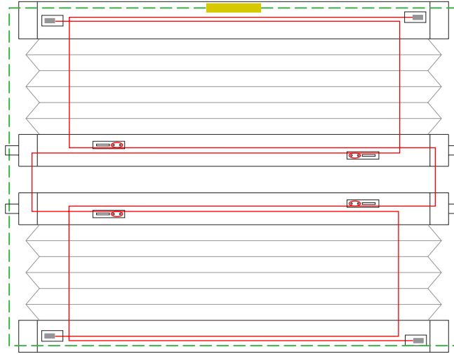
2 Schnurbohrungen/Cord boreholes/Passages de cordon ab/starting from/à partir 280 mm
